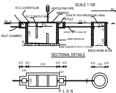
DETAILS OF SEPTIC TANK WITH SOAKPIT
