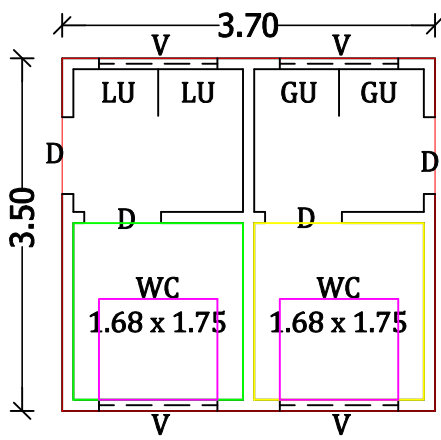
TOILET BLOCK
