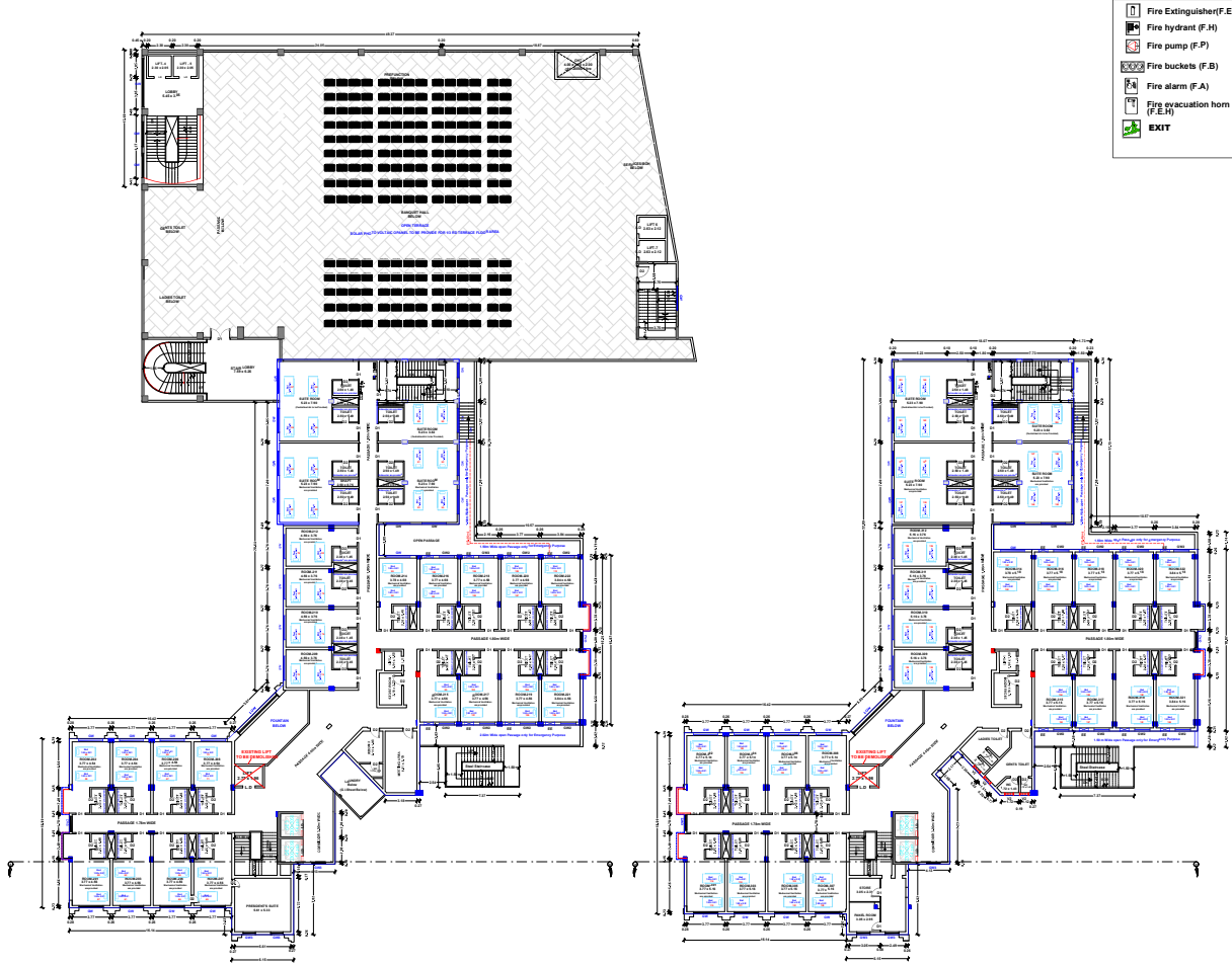
SECOND FLOOR PLAN BLOCK-A
