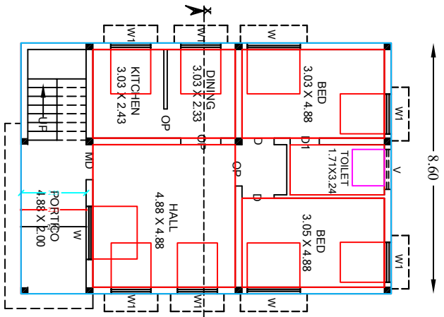
Ground Floor Plan. (Scale - 1:100)
