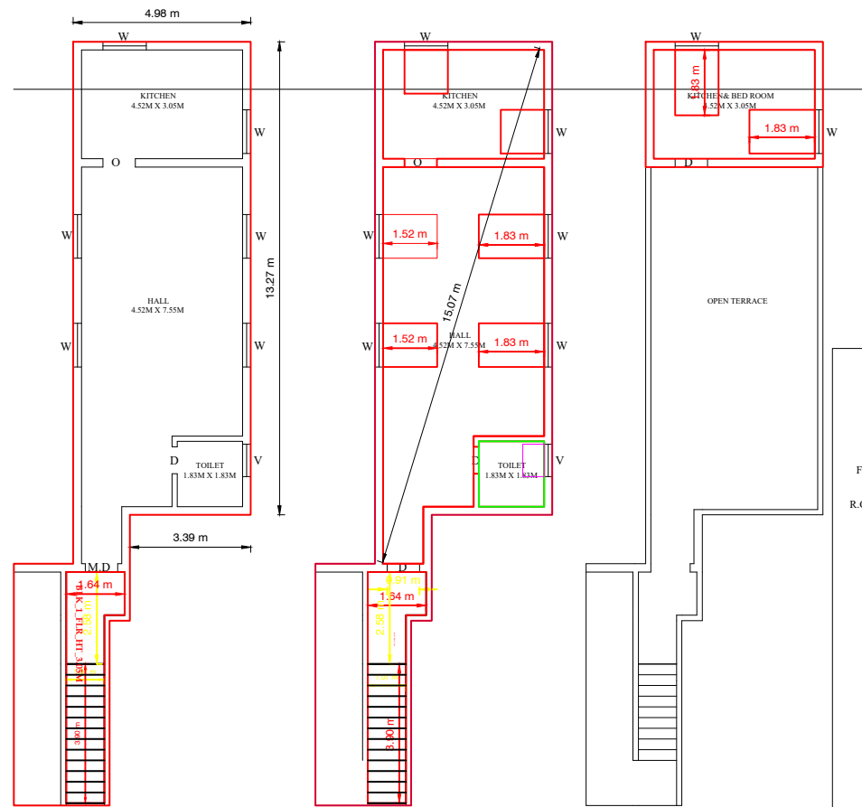
PRO S.F PLAN [NORTH FACING]
