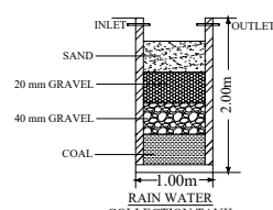
RAIN WATER COLLECTION TANK
