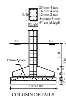
COLUMN DETAILS
