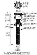
RAIN WATER HARVESTING PERCOLATION PITS
