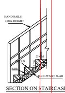
SECTION ON STAIRCASE
