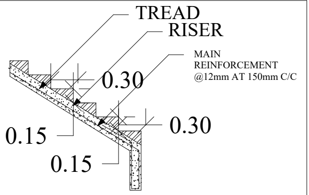
STAIRCASE DETAILS
