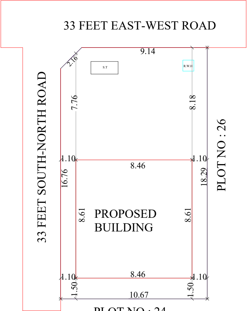
PLOT NO : 24 SITE PLAN NOT TO SCALE
