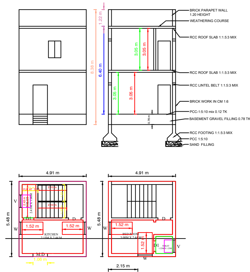
GROUND FLOOR PLAN [SOUTH FACING]
