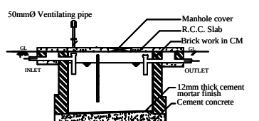
Longitudinal Section (SEPTIC TANK)
