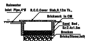
SECTION ON "MN"
