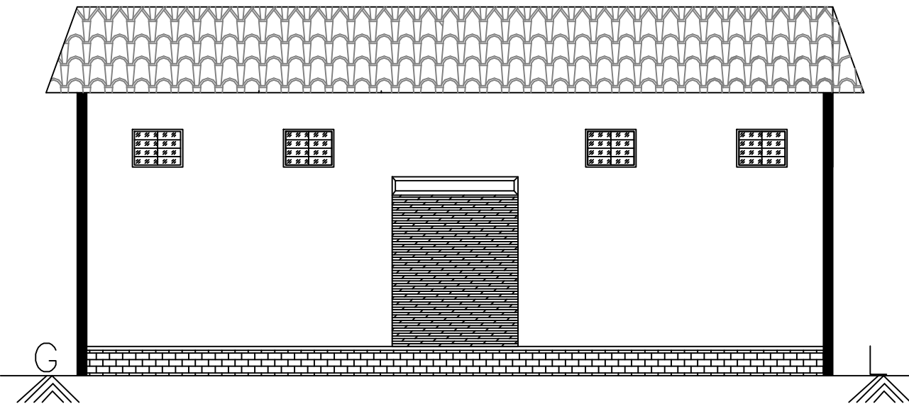
FRONT ELEVATION
