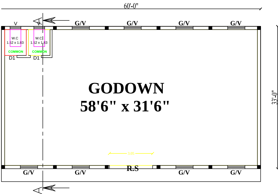
GROUND FLOOR-PLAN
