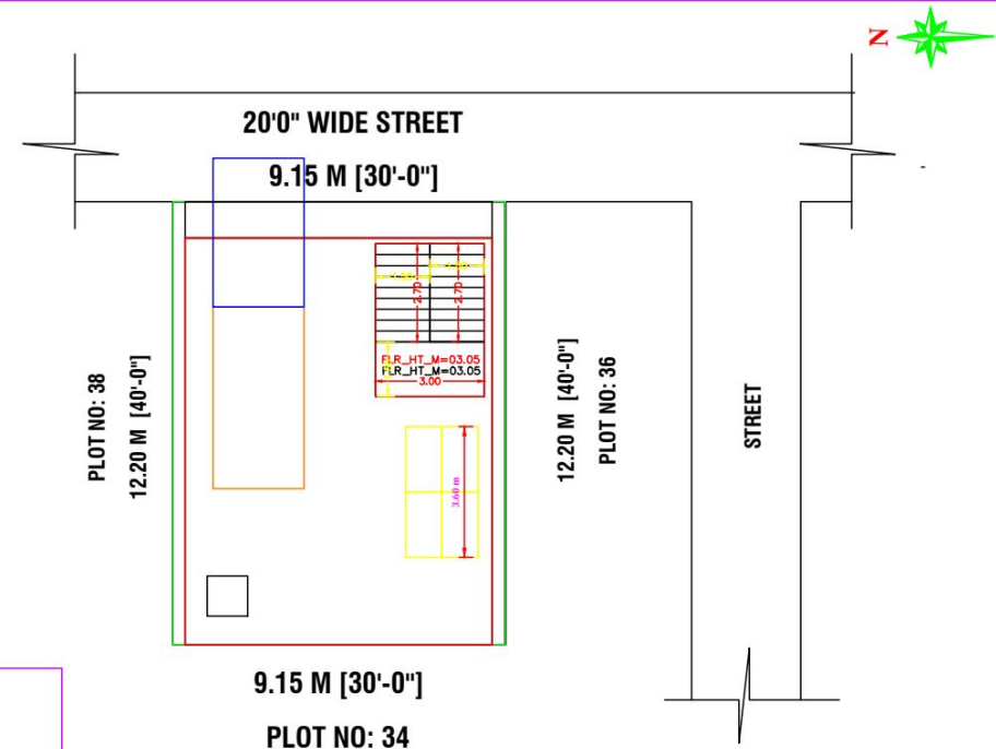
SITE PLAN
