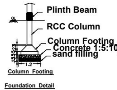
Foundation Detail
