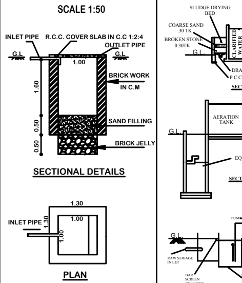
RAIN WATER COLLECTION PIT SCALE 1:50
