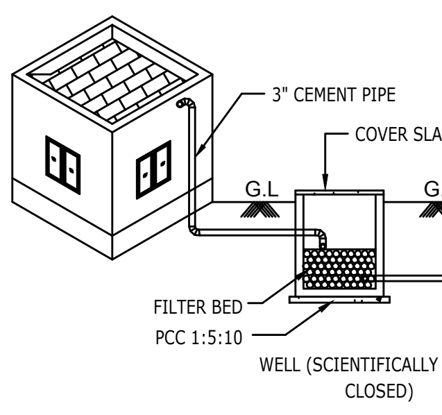
PROPOSED RAIN WATER HARVESTING CHAMBER
