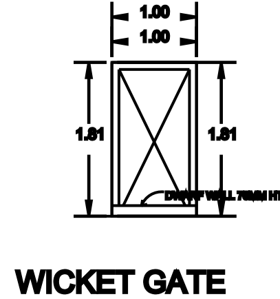
WICKET GATE
