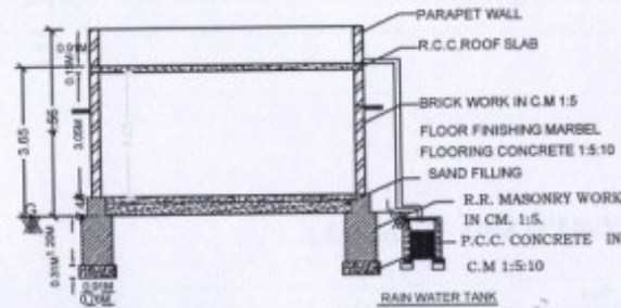
SECTION - XX
