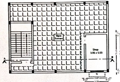
FIRST FLOOR PLAN SCALE: 1:100
