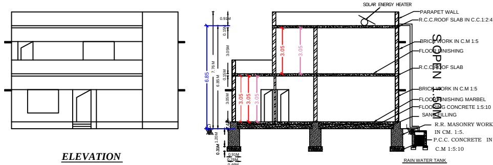
SECTION - XX
