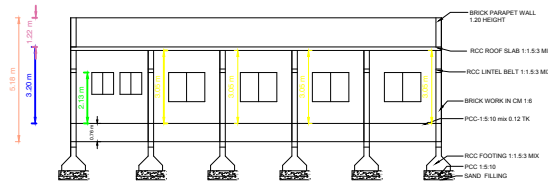
SECTION"AB"
