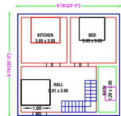
PRO.GROUND FLOOR PLAN NORTH FACING
