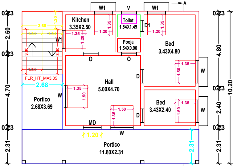
FLOOR GROUND PROPOSED GROUND FLOOR
