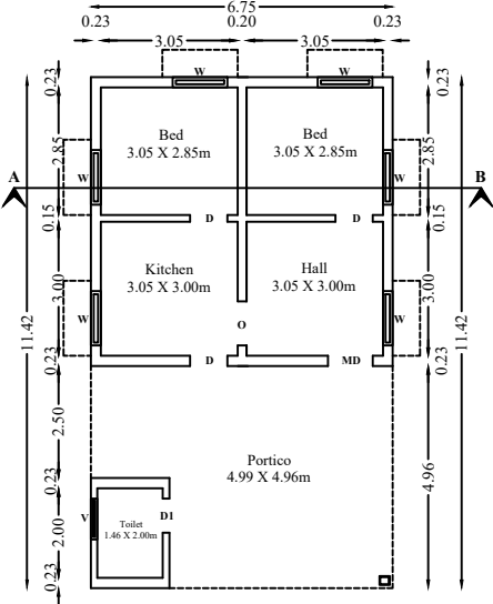
GROUND FLOOR PLAN SCALE - 1:100
