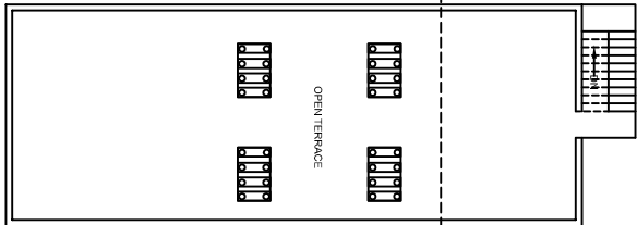
TERRACE FLOOR PLAN. (Scale - 1:100)
