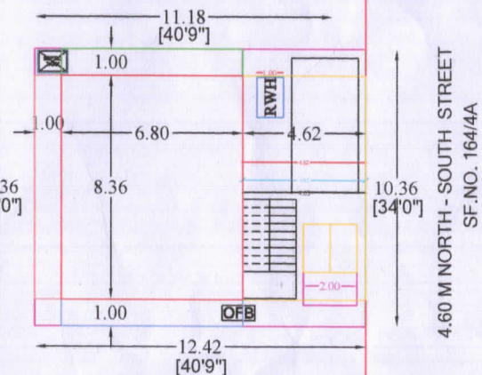
Gandhimathi House. Site Plan. (1:100)
