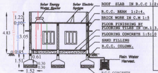
Section - XY
