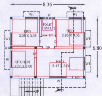
Ground Floor Plan. (Scale - 1:100)
