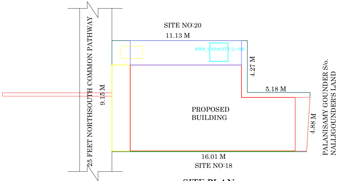
SITE PLAN
