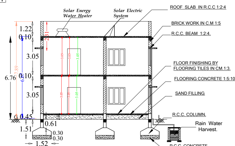
Section - XY
