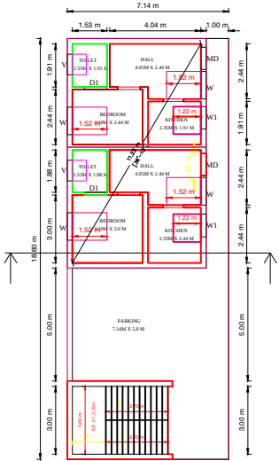
GROUND FLOOR PLAN [SOUTH FACING]
