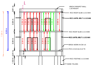
SECTION
