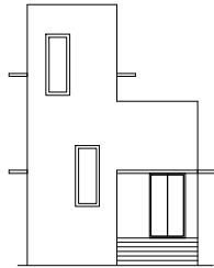
FRONT ELEVATION
