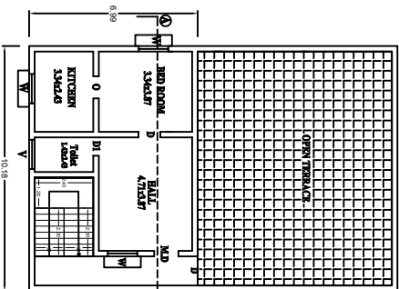
PROPOSED FIRST FLOOR
