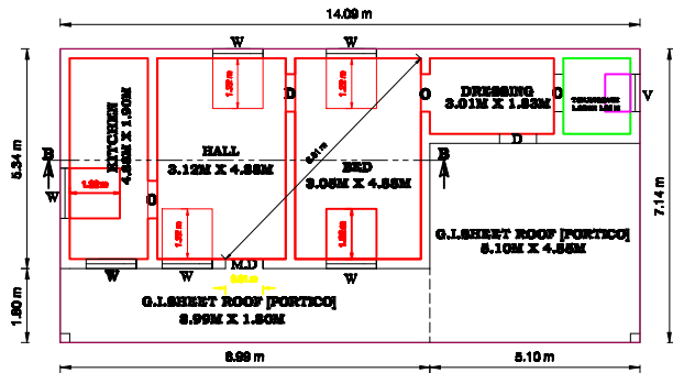
GROUND FLOOR [G.I.SHEET ROOF] - PLAN
