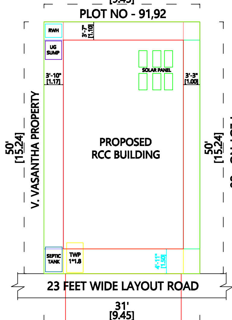
SITE PLAN (1:100)
