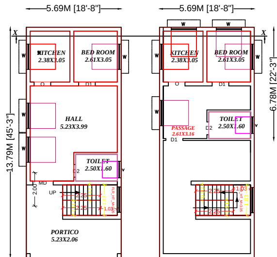
GROUND FLOOR PLAN FIRST FLOOR PLAN
