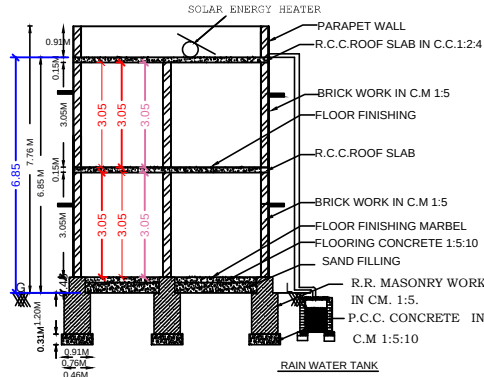
SECTION - XX
