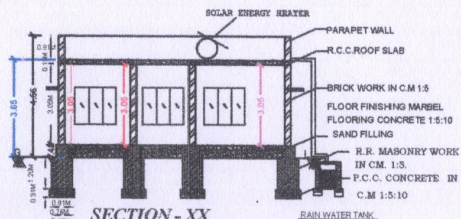
SECTION - XX
