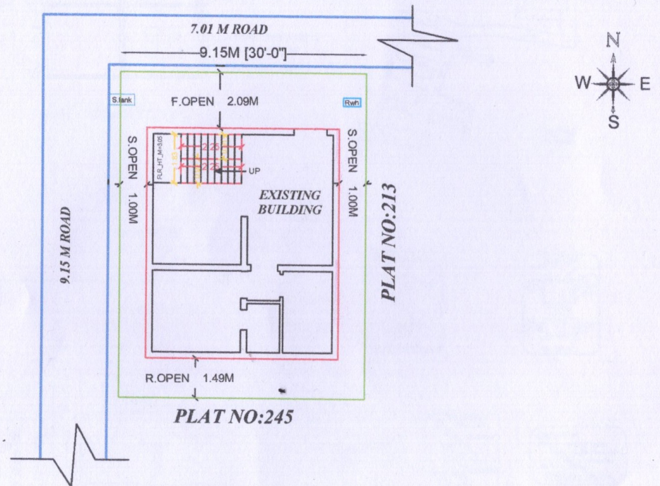
SITE PLAN
