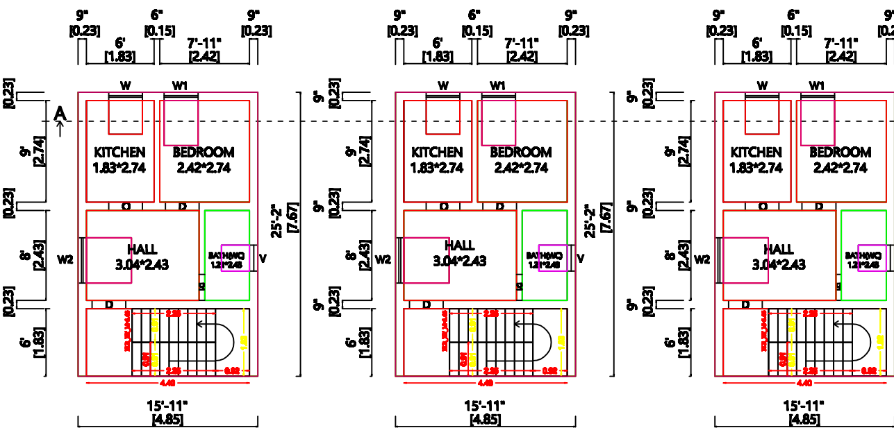
PROPOSED GROUND FLOOR PLAN PROPOSED FIRST FLOOR PLAN PROPOSED SECOND FLOOR PLAN
