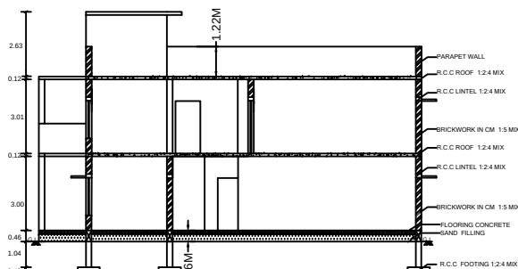
SECTION ON 'ABCD'
