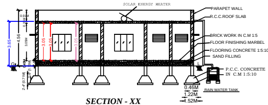
SECTION - XX
