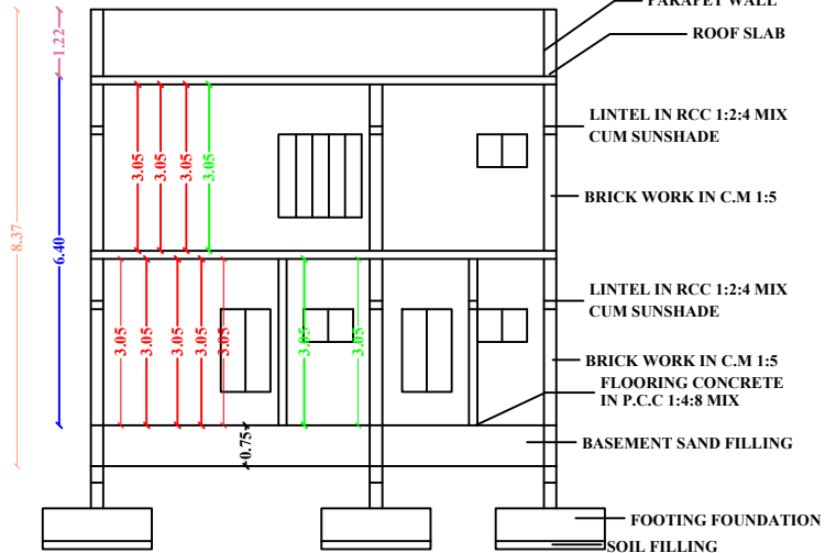
SECTION"AB"
