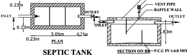
SEPTIC TANK
