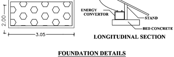
FOUNDATION DETAILS
