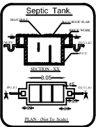
SECTION - XX
