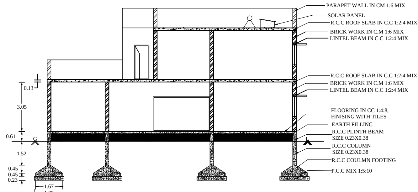
SECTION "A-B"
