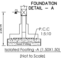
Isolated Footing -A (1.50X1.50)
