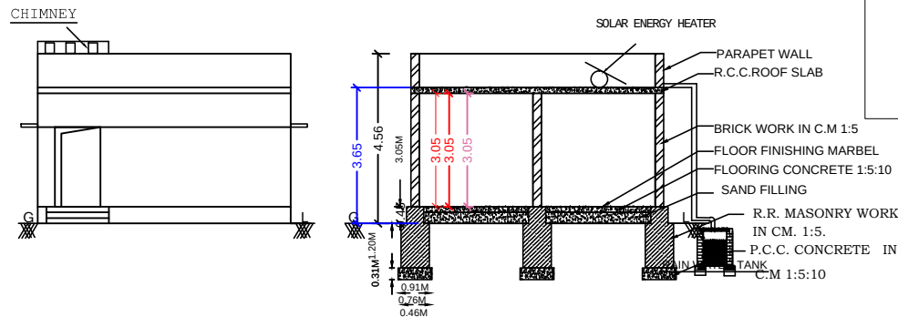
SECTION - XX
