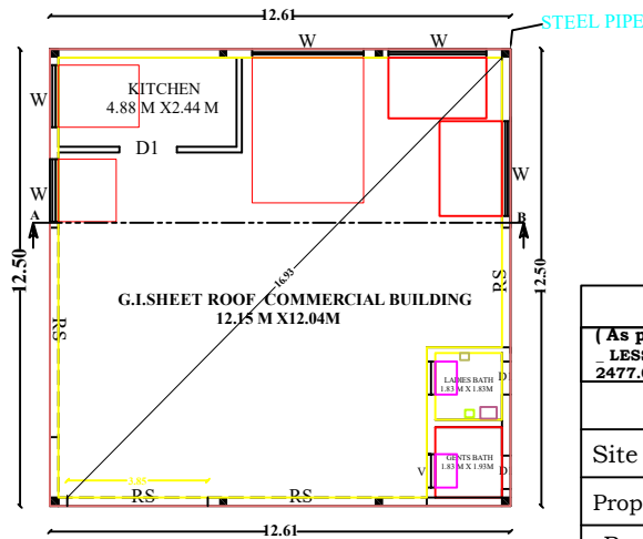
COMMERCIAL BUILDING - PLAN
