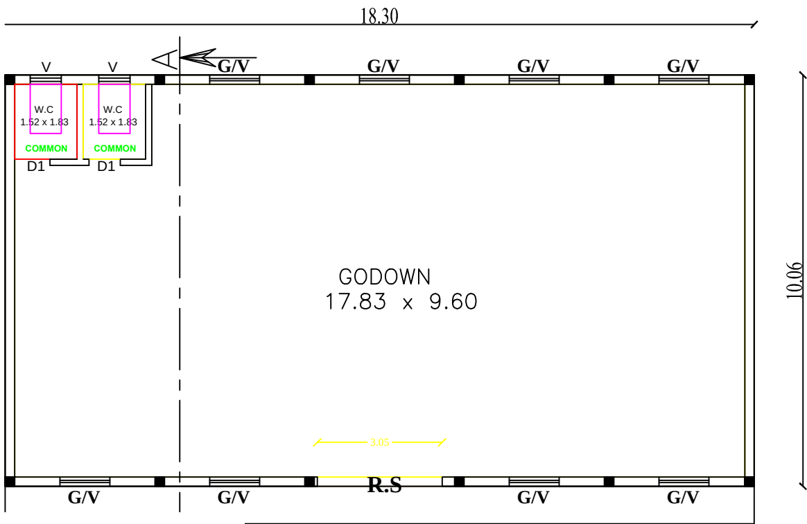
OUND FLOOR-PLAN
