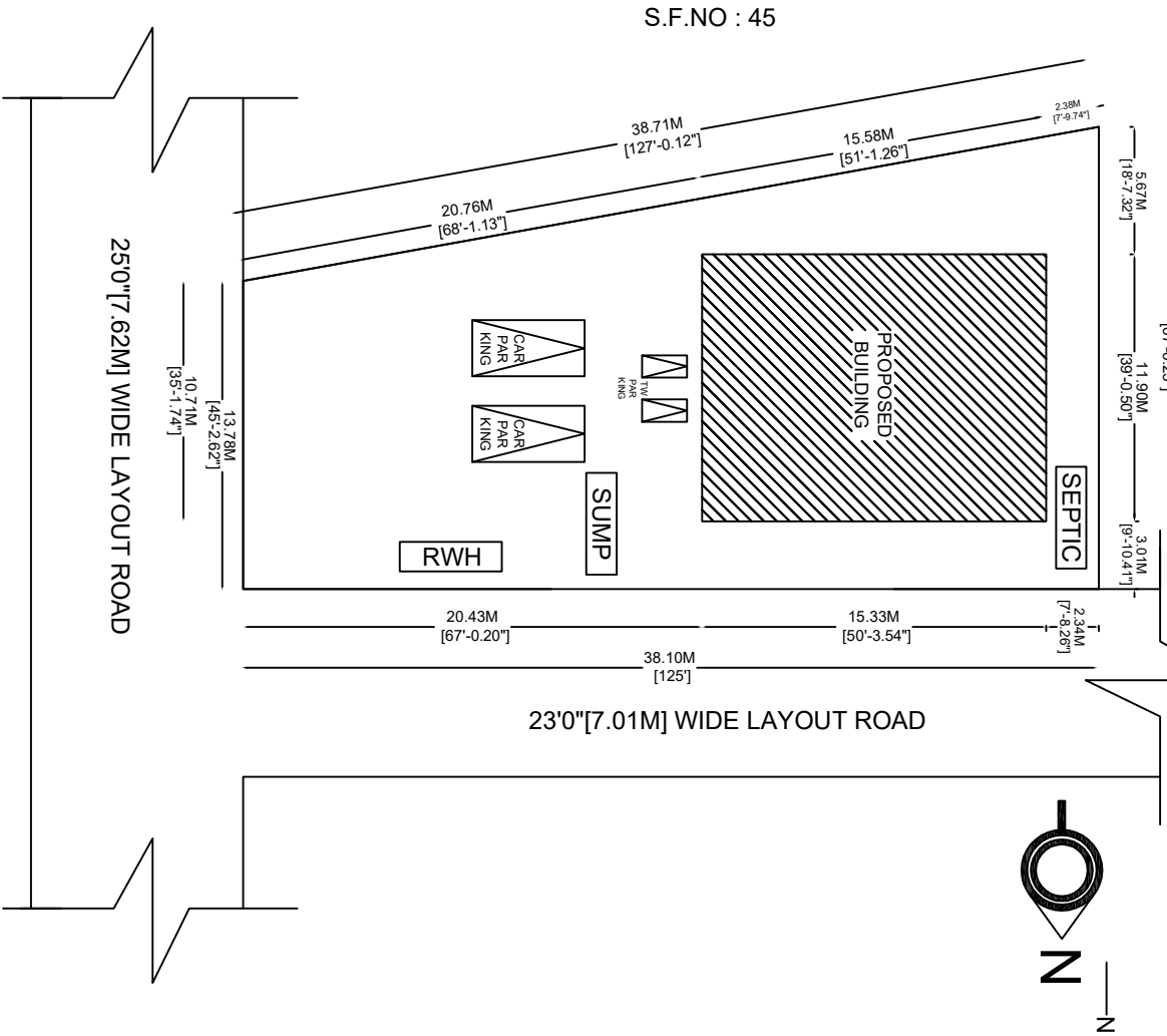
SITE PLAN
