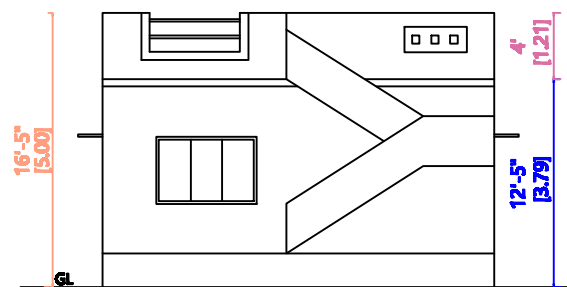
FRONT ELEVATION ( NORTH SIDE VIEW)
