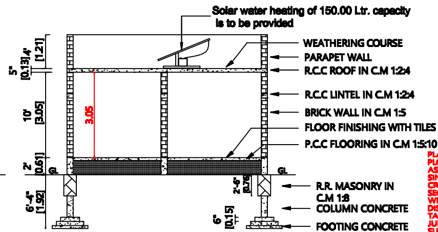
CROSS SECTION "AB"
