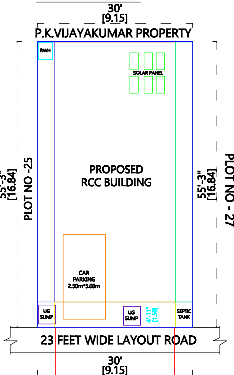
SITE PLAN (1:100)
