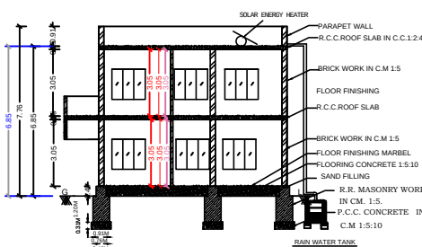
SECTION - XX
