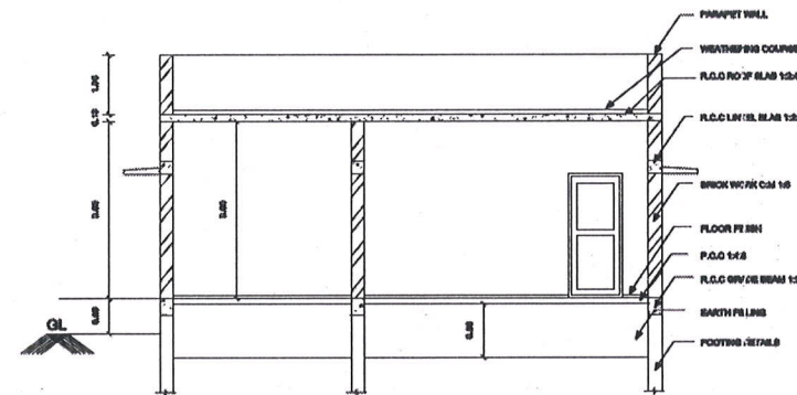
SECTION 'A-B'
