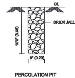
PERCOLATION PIT
