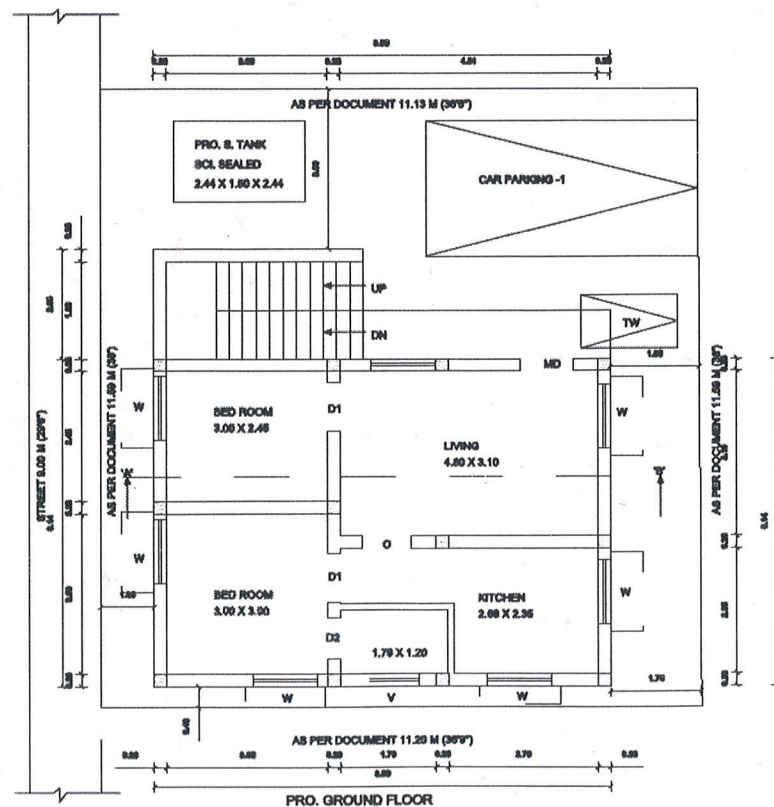
PRO. GROUND FLOOR
