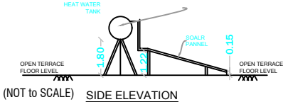
(NOT TO SCALE) SIDE ELEVATION
