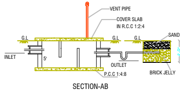
SECTION-AB
