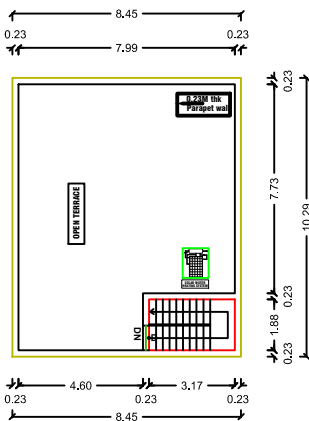
PRO.TERRACE FLOOR PLAN
