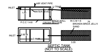
SEPTIC TANK (NOT TO SCALE)
