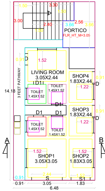
GROUND FLOOR PLAN SCALE 1 CM = 1 M
