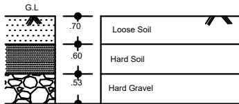
TRIAL PIT DETAILS (NOT TO SCALE)
