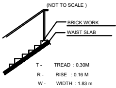
STAIR DETAILS :-
