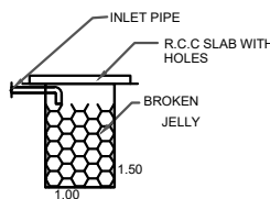
RAIN WATER HARVESTING FILTER BED
